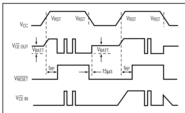
Figure 6. Chip-Enable Timing
