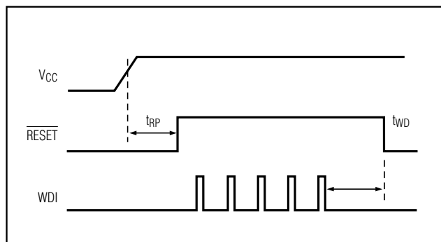
Figure 4. Watchdog Timing
