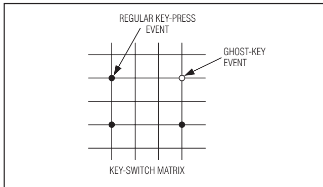
Figure 9. Ghost-Key Phenomenon
