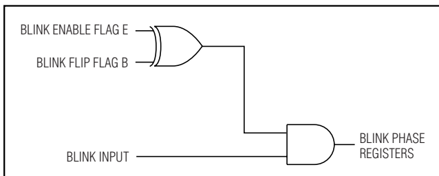
Figure 11. BLINK Logic
