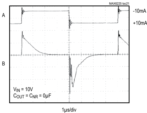
LOAD-TRANSIENT RESPONSE
