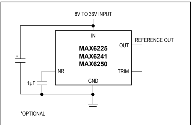
Figure 2. Noise-Reduction Capacitor
