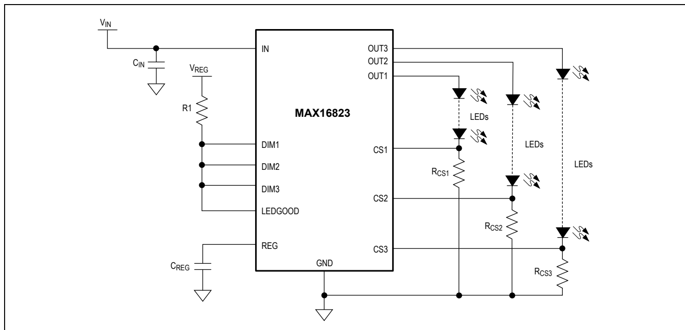
Figure 3. Output_Latch-Off
