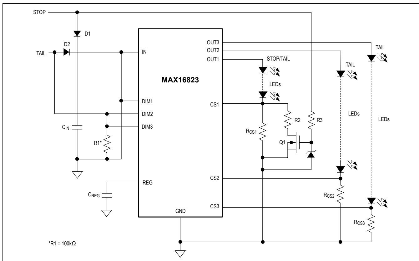
Figure 4. Two-Brightness Level with Current Level Switch for TAIL/STOP Lights
