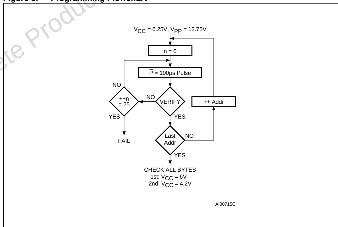
Figure 5. Programming Flowchart
