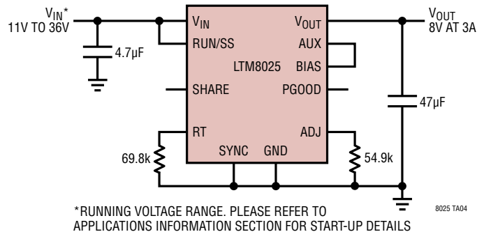
8V Step-Down Converter
