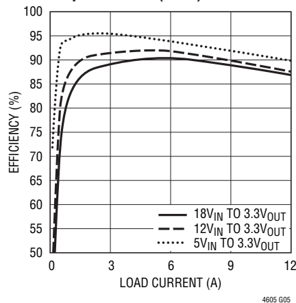
Efficiency vs Load Current 1.5μH Inductor (CCM)
