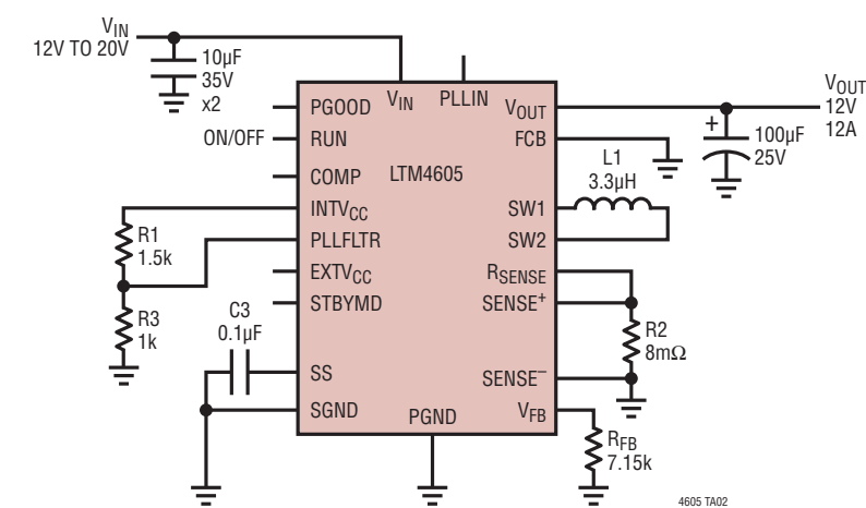
Figure 14. Buck Mode Operation with 12V to 20V Input
