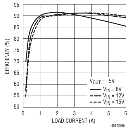
Figure 19. Buck Mode Operation with Positive Input to Negative -5V Output Converter
