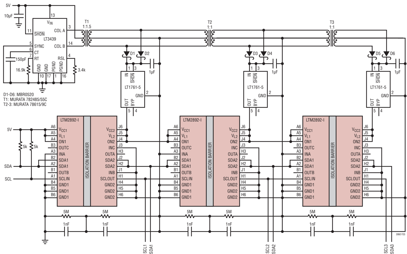
Figure 31. Series Multi-Zone Isolated I²C Interface, Working Voltage Multiplier
