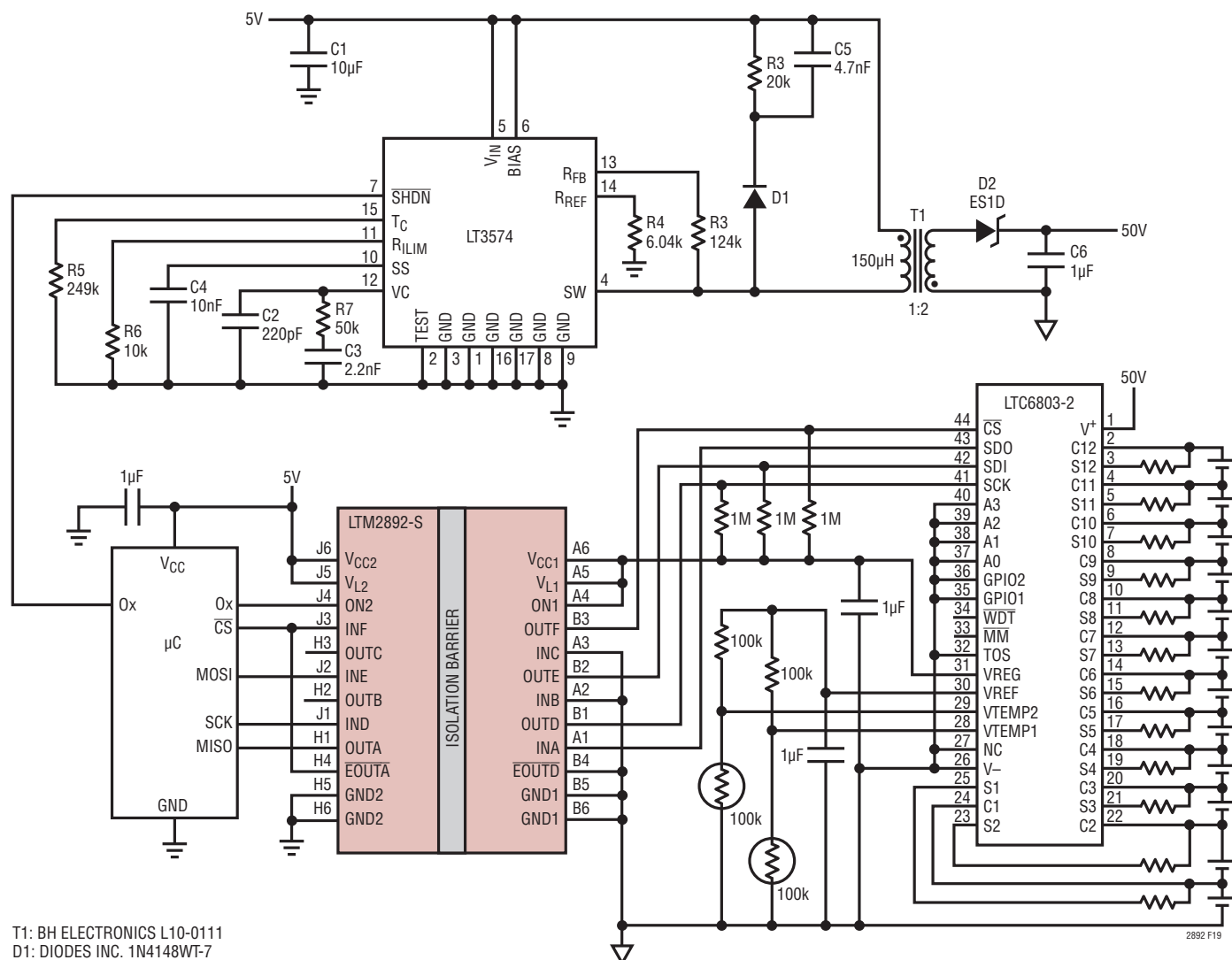
Figure 27. Battery Stack Monitor with Isolated SPI Interface
