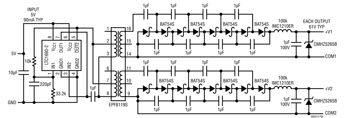
Figure 26. LTC6803 Powered by Isolated Power Supplies
