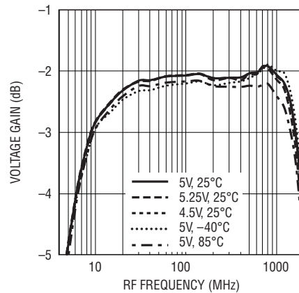
Voltage Gain vs RF Frequency
