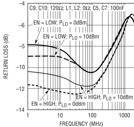
Figure 5. LO Port Return Loss vs Frequency Optimized for Low Frequency (See Figure 10)
