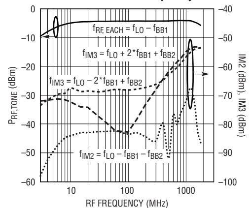
RF Two-Tone Power (Each Tone), IM2 and IM3 vs RF Frequency
