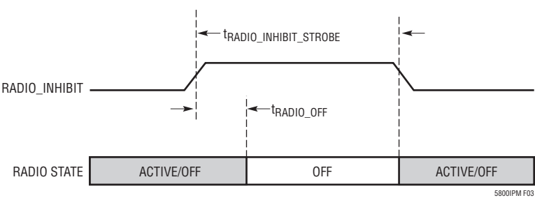
Figure 3. RADIO_INHIBIT Timing
