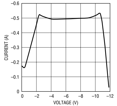
V EEOUT Current vs V EEOUT Voltage
