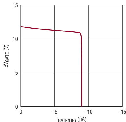
Gate Voltage vs Gate Pull-Up Current
