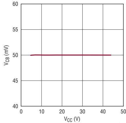
Circuit Breaker Voltage vs Supply Voltage
