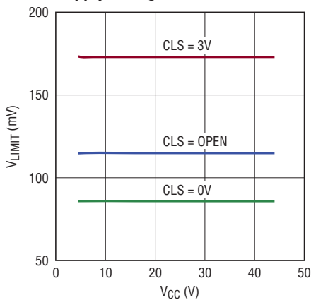
Current Limit Voltage vs Supply Voltage
