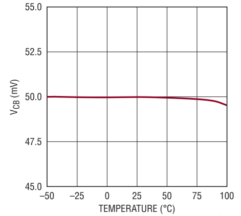
Circuit Breaker Voltage vs Temperature
