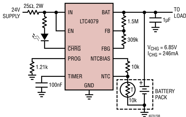
Figure 8. LiFePO 4 Charger with Timer Termination
