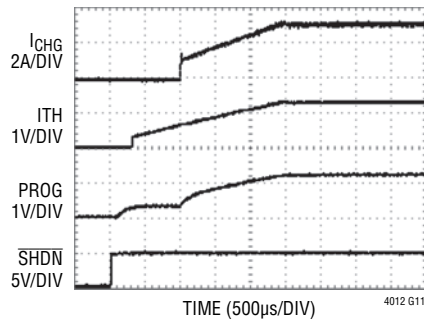
PWM Soft-Start
