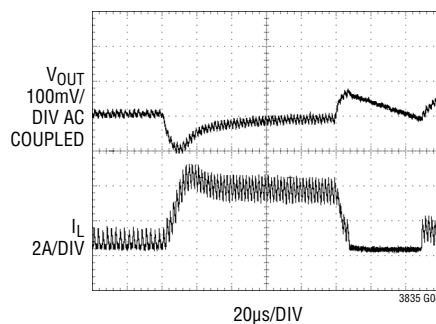
FIGURE 11 CIRCUIT V_{OUT} = 3.3\text{V}
