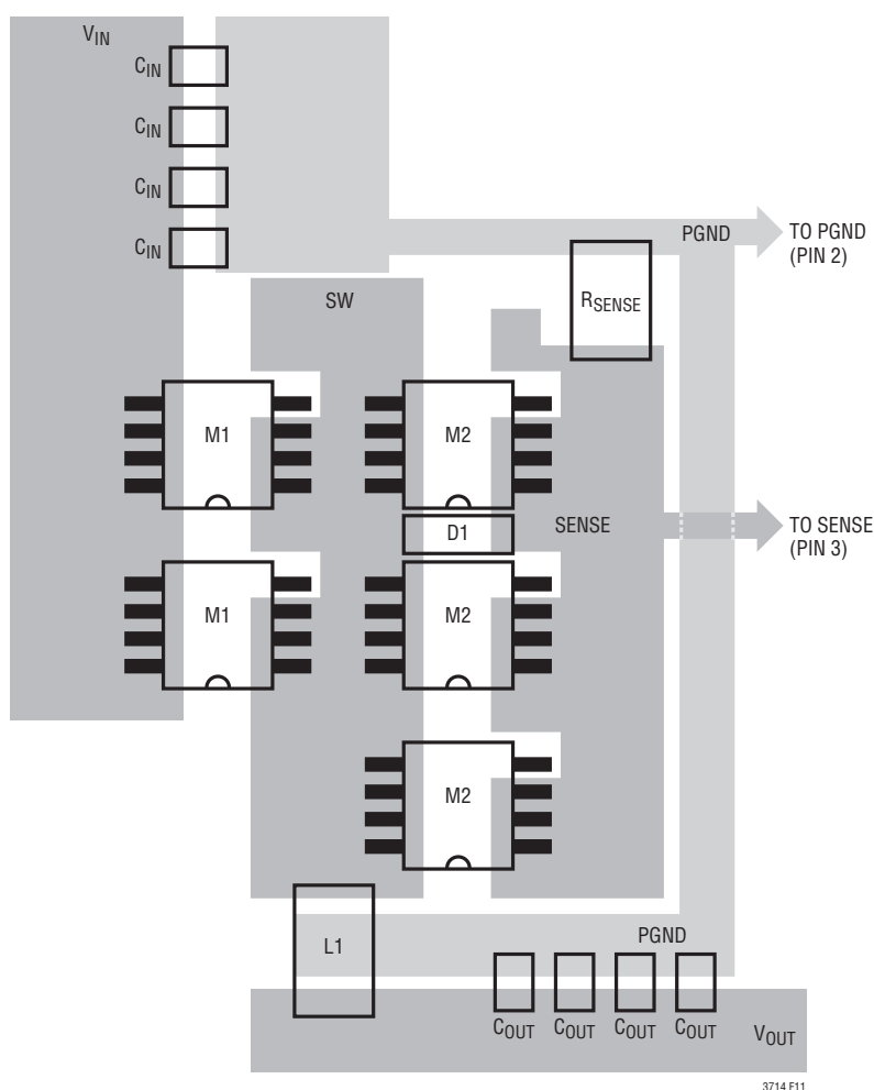
Figure 11. General Layout of External Power Components
