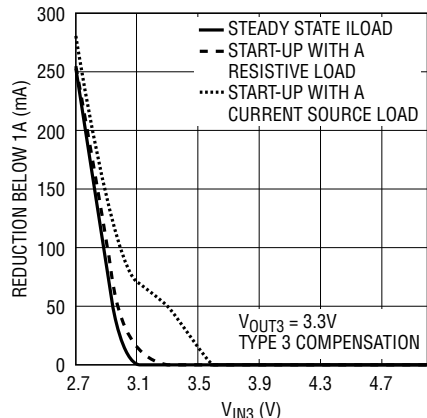
Reduction in Current Deliverability at Low V_{IN3}
