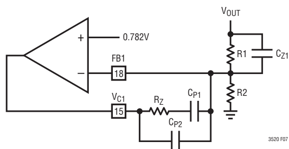
Figure 7. Type III Compensation Network
