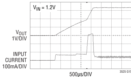
LTC3525-3.3 Input Current and V_{OUT} at Start-Up
