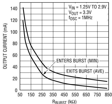
Burst Mode Output Current Threshold vs R_{\text{BURST}} (3.3V Output)
