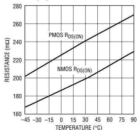
R_{\text{DS(ON)}} vs Temperature
