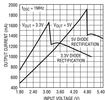
Maximum Output Current vs V_{\text{IN}}
