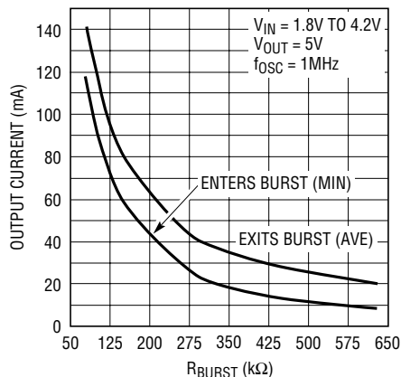
Burst Mode Output Current Threshold vs R_{\text{BURST}} (5V Output)
