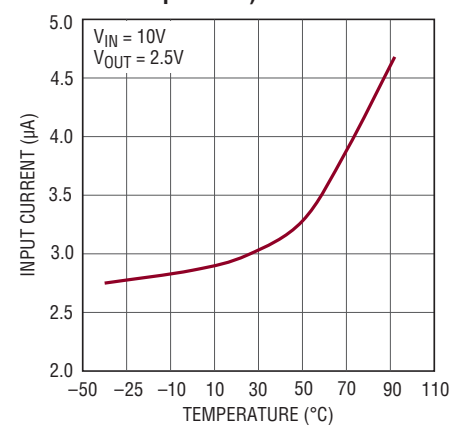
Application No-Load Input Current vs Temperature (Automatic Burst Mode Operation)
