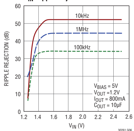
V_{IN} Ripple Rejection
