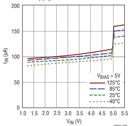
IN Supply Current
