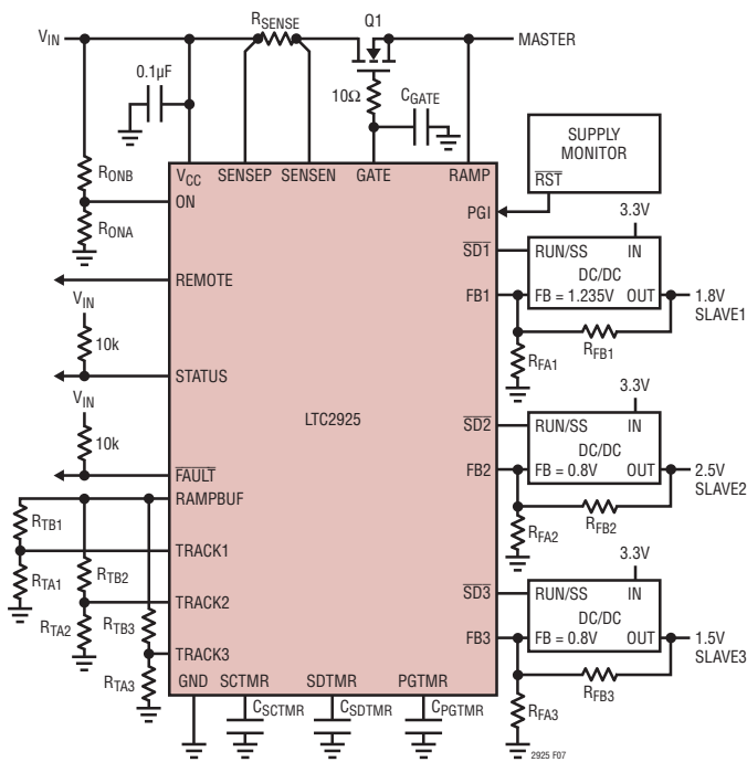
Figure 7. Typical Application with External FET
