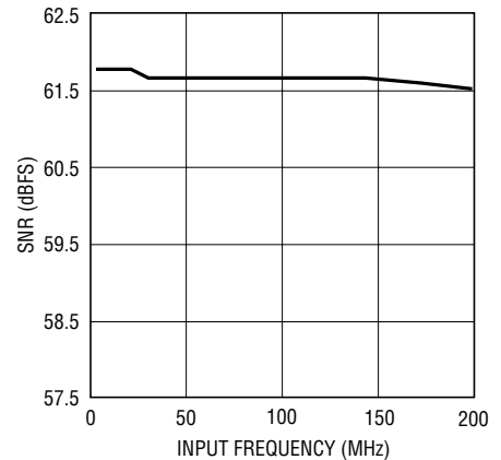
LTC2237: SNR vs Input Frequency, -1\text{dB} , 2V Range, 40Msps
