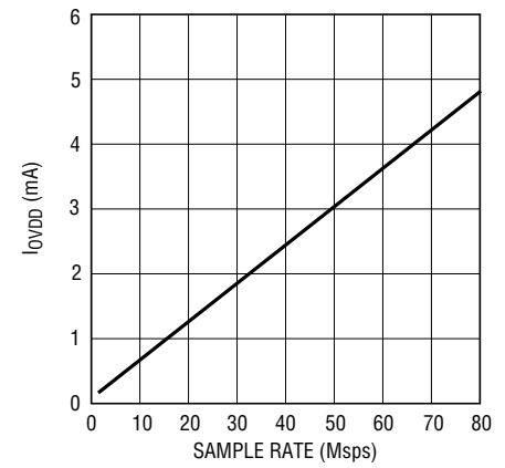
LTC2238: I_{VDD} vs Sample Rate, 5MHz Sine Wave Input, -1dB, V_{DD} = 1.8\text{V}
