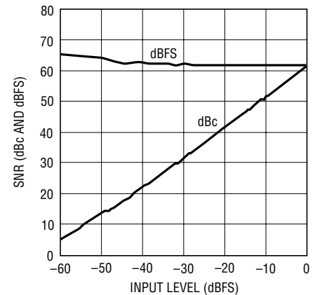
LTC2237: SNR vs Input Level, f_{IN} = 5\text{MHz} , 2V Range, 40Msps
