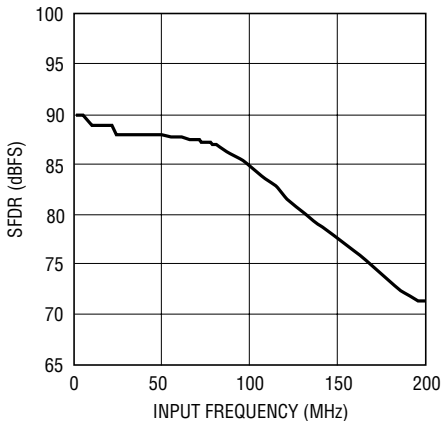
LTC2237: SFDR vs Input Frequency, -1\text{dB} , 2V Range, 40Msps
