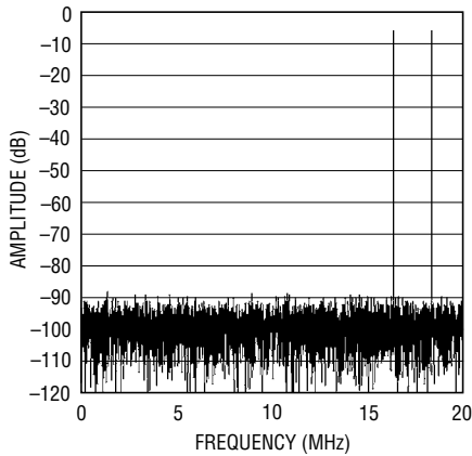
LTC2237: 8192 Point 2-Tone FFT, f_{IN} = 21.6\text{MHz} and 23.6\text{MHz} , -1\text{dB} , 2V Range, 40Msps
