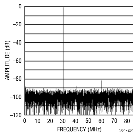
LTC2220: 8192 Point FFT, f_{IN} = 140\text{MHz} , -1\text{dB} , 1V Range, LVDS Mode
