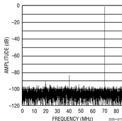
LTC2220: 8192 Point FFT, f_{IN} = 70\text{MHz} , -1\text{dB} , 2V Range, LVDS Mode
