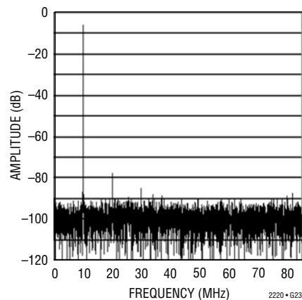
LTC2220: 8192 Point FFT, f_{IN} = 500\text{MHz} , -6\text{dB} , 1V Range, LVDS Mode
