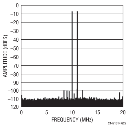
LTC2141-14: 64k Point 2-Tone FFT, f_{IN} = 69\text{MHz} , 70MHz, -7\text{dBFS} , 40Msps
