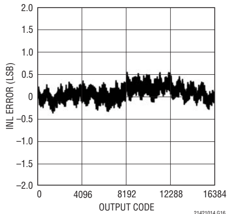
LTC2141-14: Integral Nonlinearity (INL)
