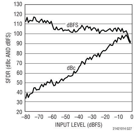
LTC2141-14: SFDR vs Input Level, f_{IN} = 70\text{MHz} , 40Msps, 2V Range
