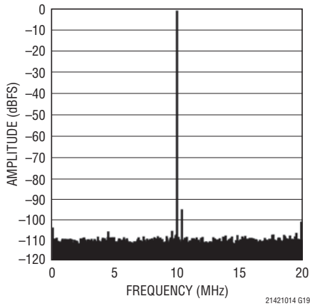
LTC2141-14: 64k Point FFT, f_{IN} = 30\text{MHz} , -1\text{dBFS} , 40Msps
