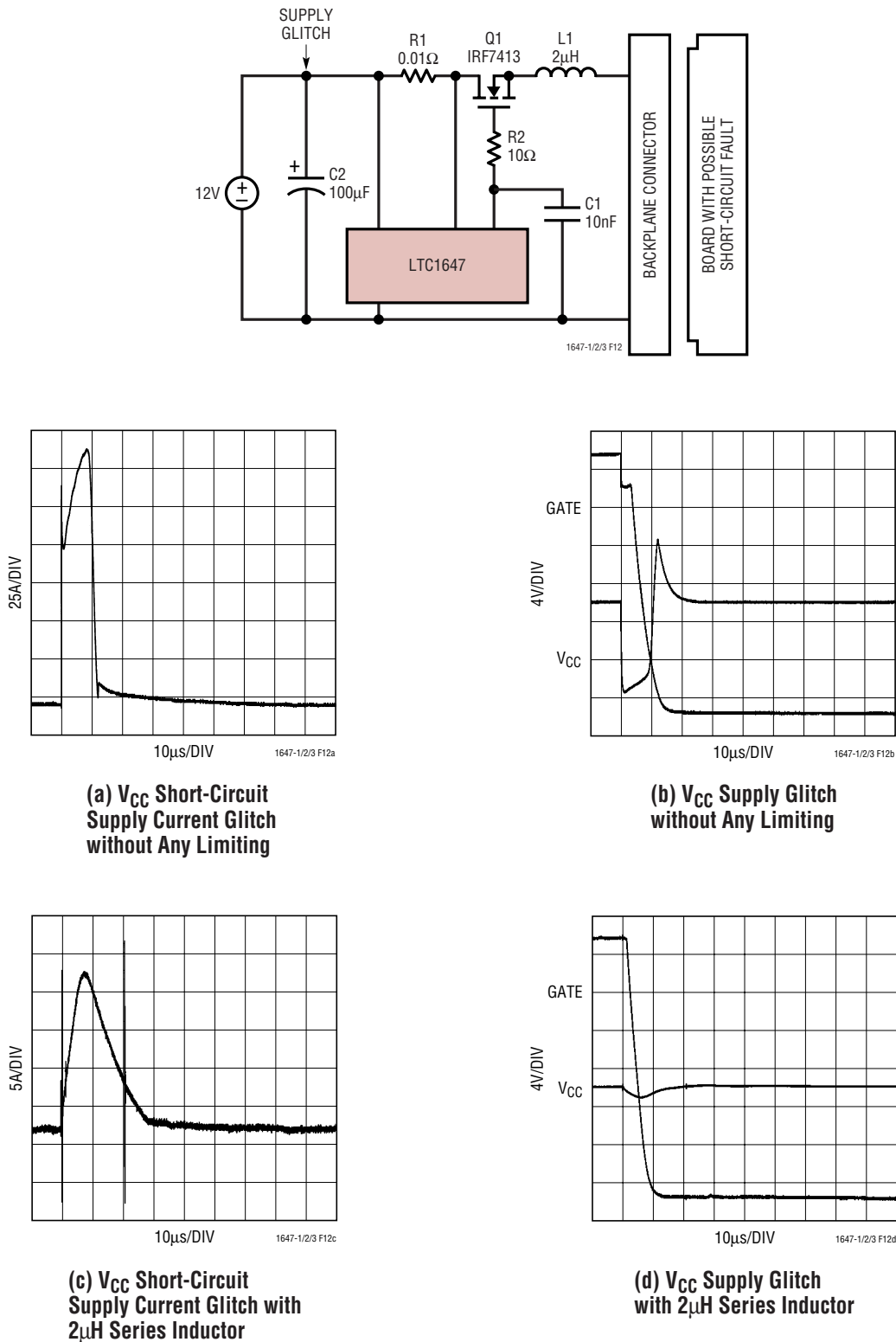
Figure 12. Supply Glitch
