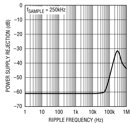
Power Supply Rejection vs Ripple Frequency
