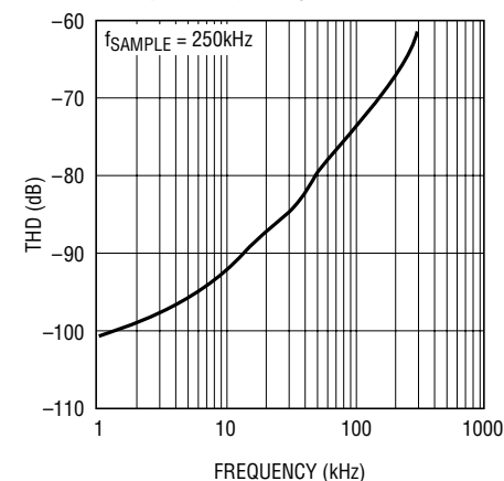
Total Harmonic Distortion (THD) vs Input Frequency
