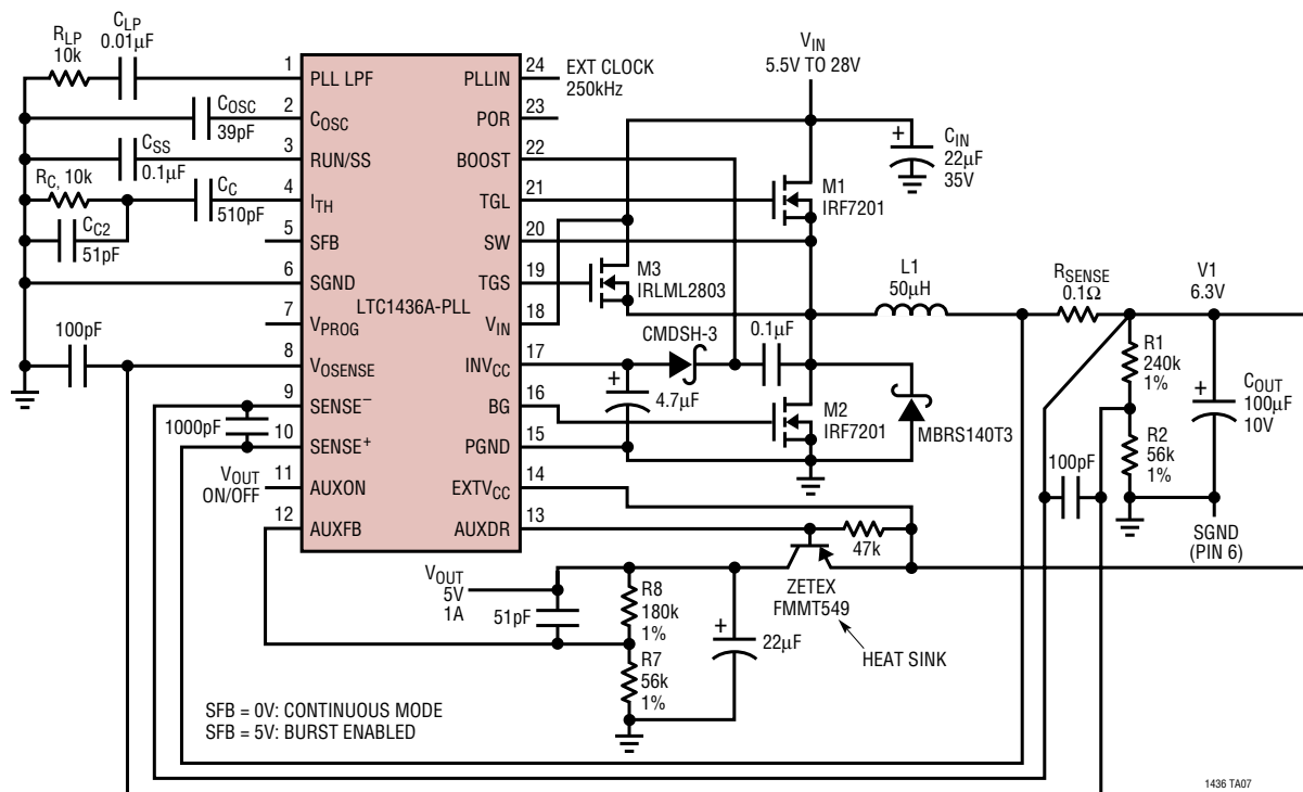
LTC1436A-PLL Low Noise High Efficiency 5V/1A Regulator
