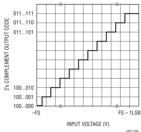
Figure 5. LTC1407-1/LTC1407A-1 Transfer Characteristic
