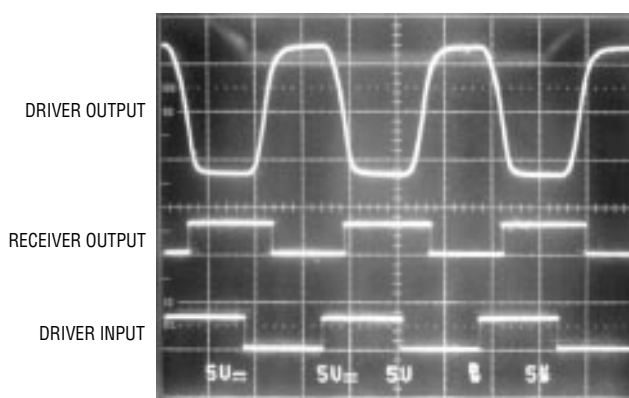
Figure 6. Driver Test Result at 120kbaud
