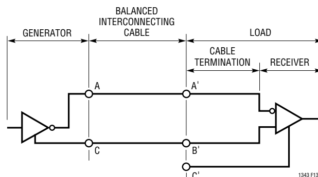
Figure 13: Typical V.10 Interface
