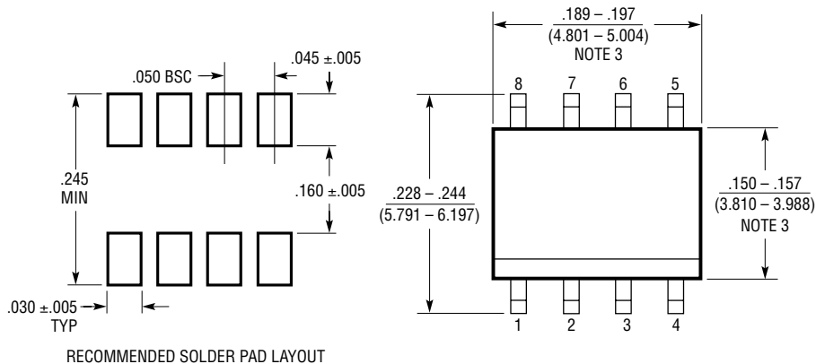
RECOMMENDED SOLDER PAD LAYOUT
