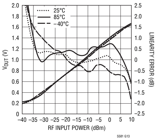
Output Voltage and Linearity Error at 2600MHz
