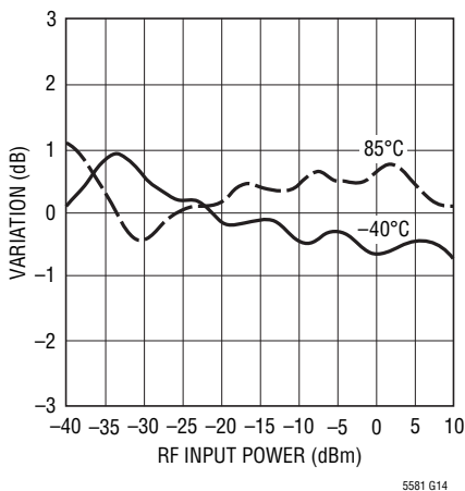
Linearity Error Temperature Variation from 25°C at 2600MHz
