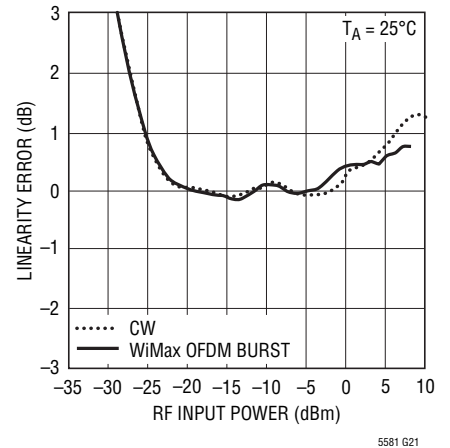
Linearity Error vs RF Input Power, 5.8GHz Modulated Waveforms
