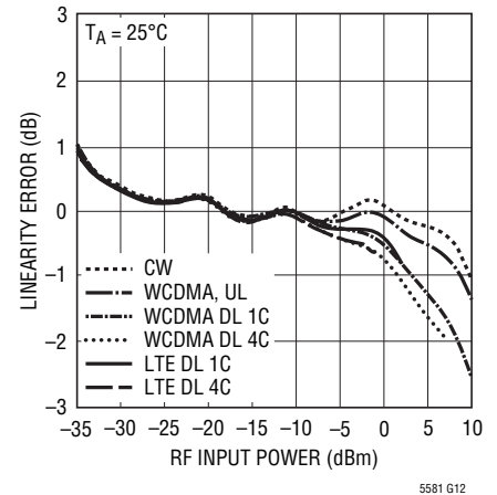
Linearity Error vs RF Input Power, 2.6GHz Modulated Waveforms
