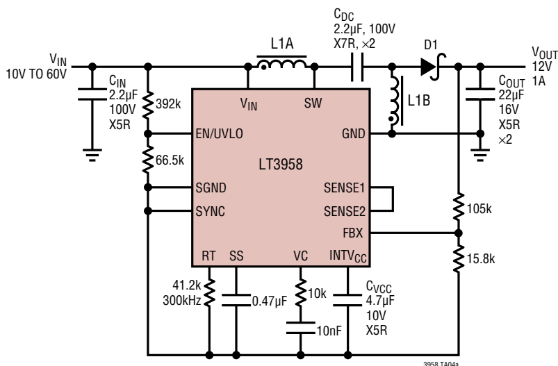
10V to 60V Input, 12V Output SEPIC Converter
