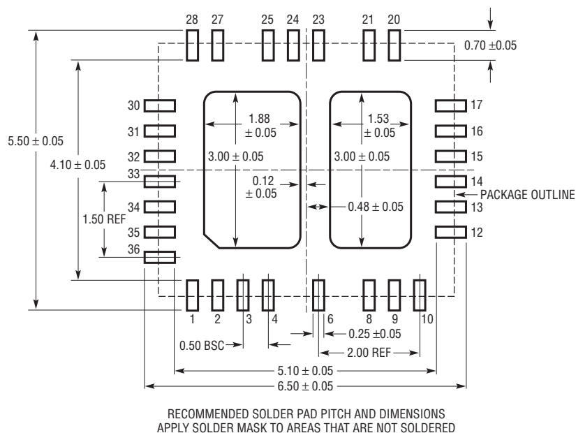
UHE Package Variation: UHE36(28)MA 36(28)-Lead Plastic QFN (5mm × 6mm) (Reference LTC DWG # 05-08-1836 Rev D)
