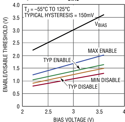
Enable Pin Threshold and Hysteresis vs V_{BIAS}
