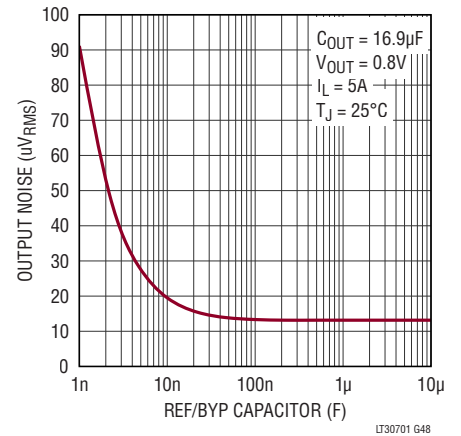
RMS Output Noise vs CREF/BYP
