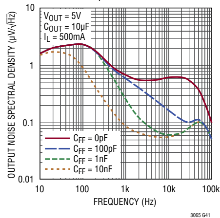
Output Noise Spectral Density vs C_{FF} , C_{REF/BYP} = 10\text{nF}
