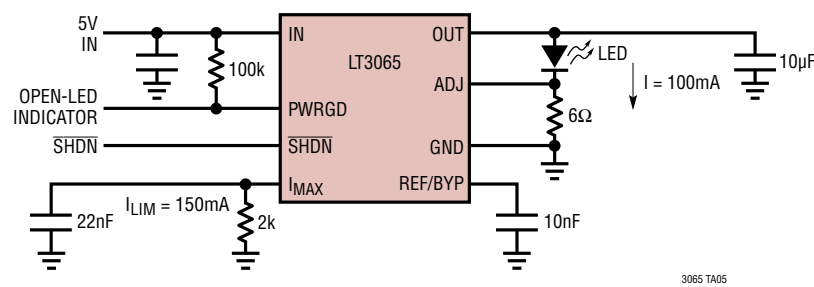
LED Driver/Current Source
