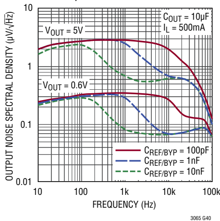
Output Noise Spectral Density vs C_{REF/BYP} , C_{FF} = 0
