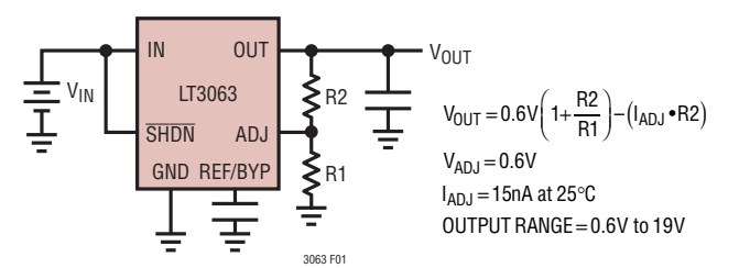
Figure 1. Adjustable Operation
