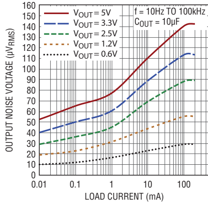
RMS Output Noise vs Load Current C_{\text{REF/BYP}} = 10\text{nF} , C_{\text{FF}} = 0
