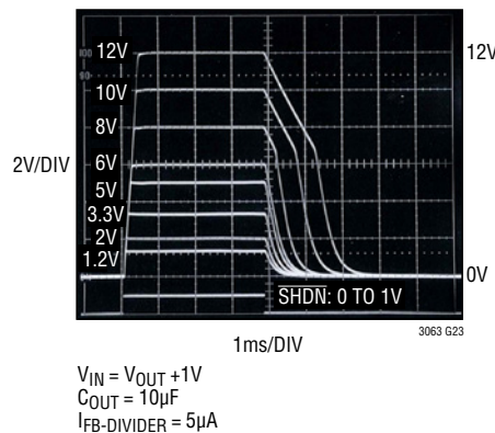
Output Discharge vs V_{OUT} C_{REF/BYP} = 0
