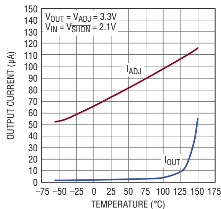
Reverse Current
