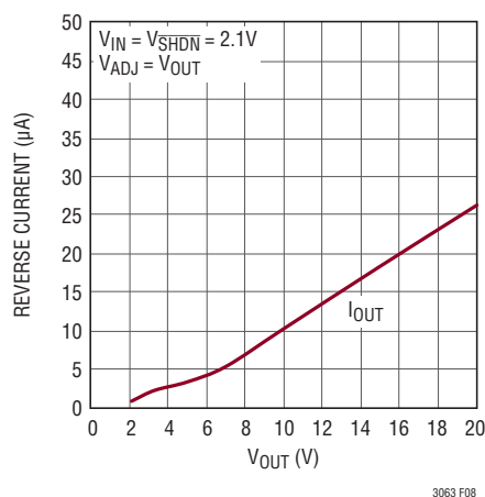
Figure 8. LT3063 Reverse Output Current
