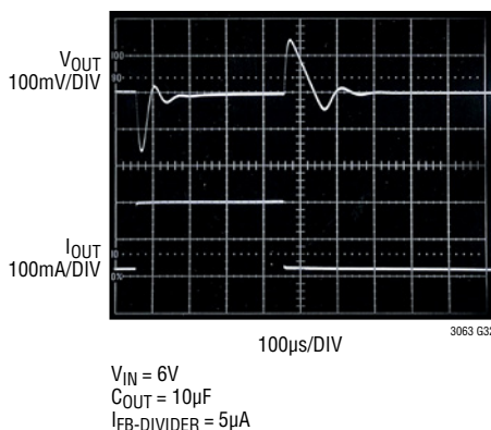
5V Transient Response C_{FF} = 0 , I_{OUT} = 20mA \text{ to } 200mA
