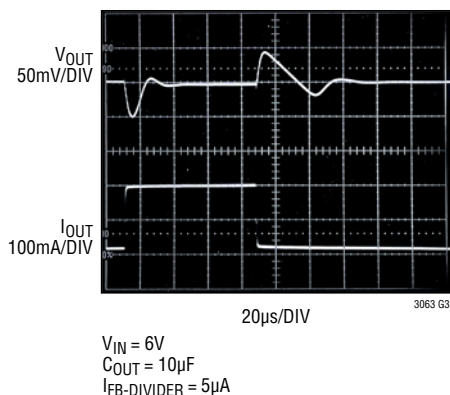
5V Transient Response C_{FF} = 10nF , I_{OUT} = 20mA \text{ to } 200mA
