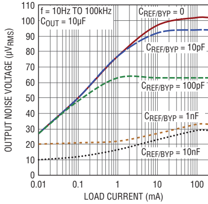
RMS Output Noise vs C_{\text{REF/BYP}} , V_{\text{OUT}} = 0.6\text{V}
