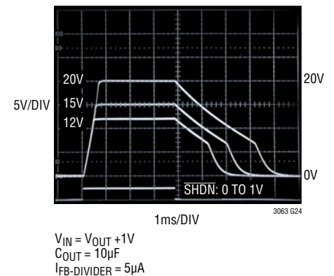
Output Discharge vs V_{OUT} C_{REF/BYP} = 0
