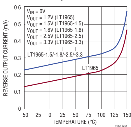
Reverse-Output Current
