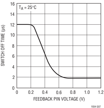
Frequency Foldback
