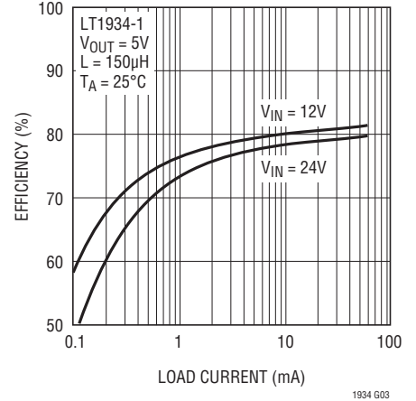
LT1934-1 Efficiency, V_{OUT} = 5V
