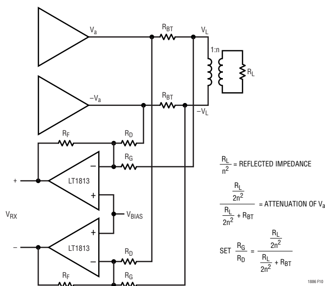
Figure 10. Receiver Configuration
