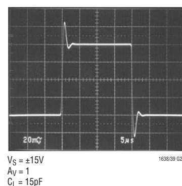
Small-Signal Response
