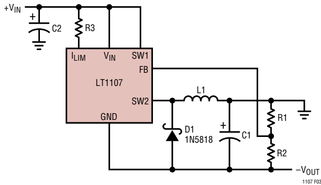
Figure 3. Positive-to-Negative Converter
