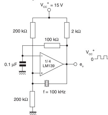
Figure 19. Crystal-controlled oscillator
