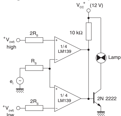
Figure 18. Limit comparator
