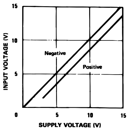
Figure 6. Input voltage range
