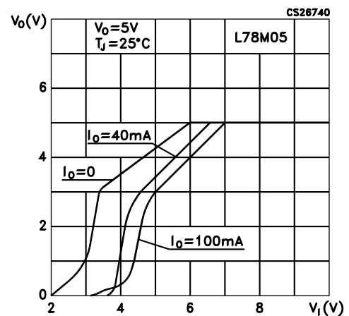
Figure 9. Dropout characteristics
