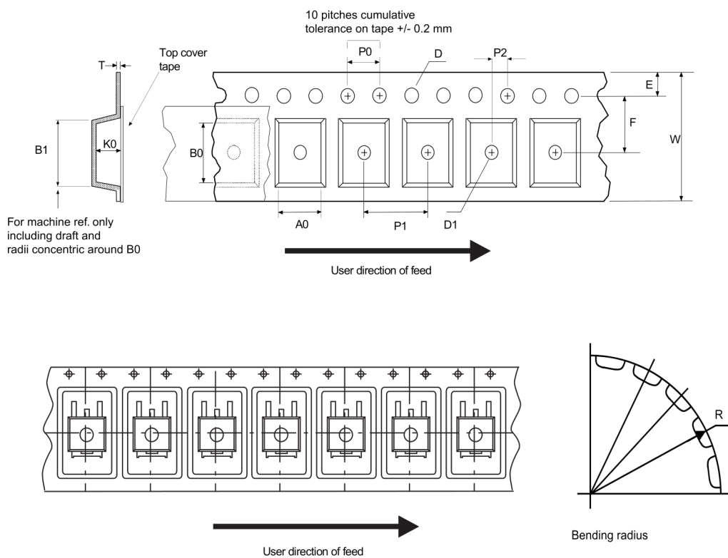
Figure 36. DPAK tape
