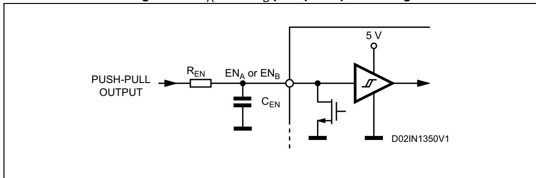
Figure 8. EN_A and EN_B pins push-pull driving
